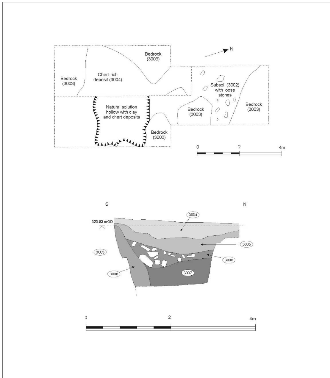
Figure 16. Plan of Trench 3 and section drawing of the solution hollow.
