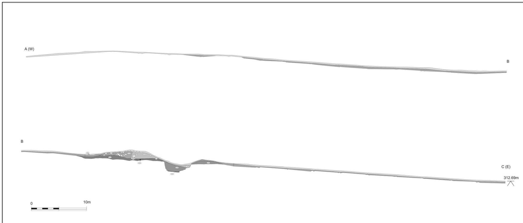
Figure 6. Section across the site showing the thickness of overburden and depth of bedrock extrapolated from observations in test pits and trench 1
