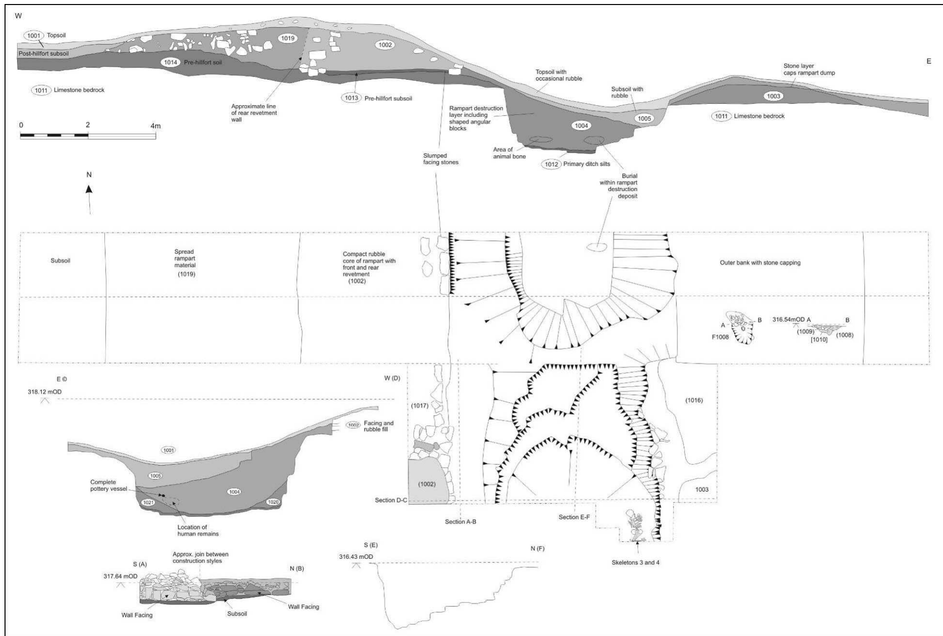
Figure 13. Plan and sections of Trenches 1a and 1b (combined).
